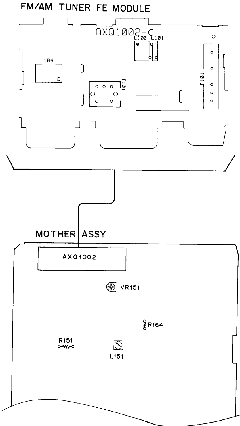
Fig. 1-2. Adjustment Points
